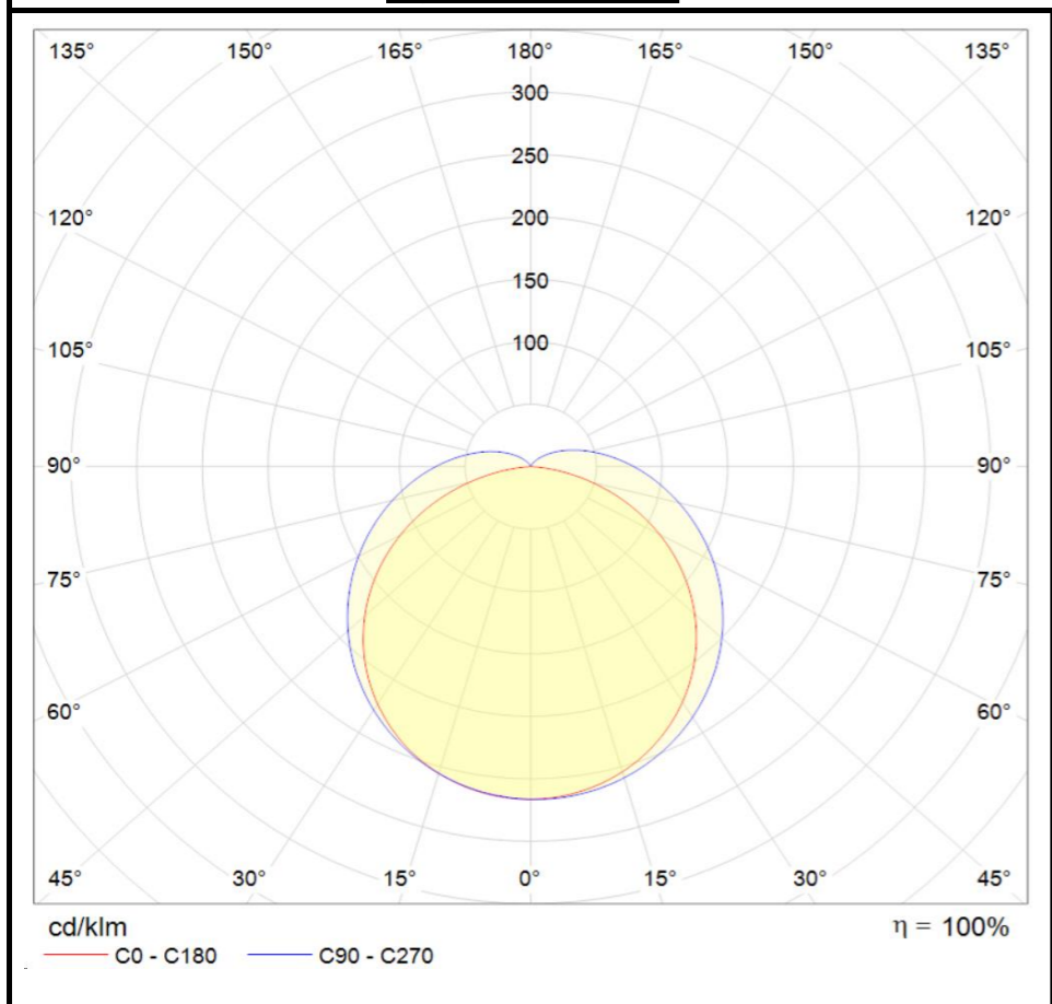
Light distribution
