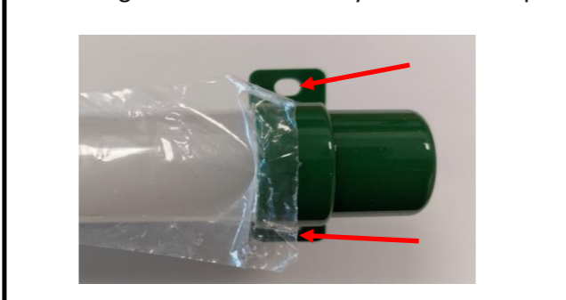
Mounting with 2 screws directly on both endcaps
